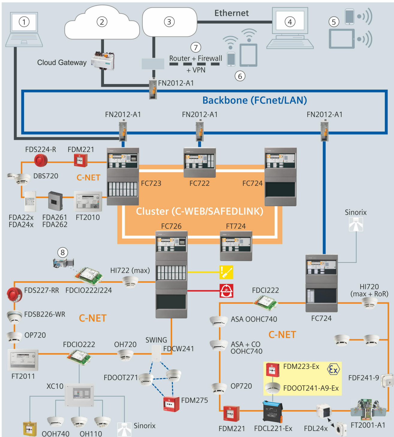
Fig. 1: System overview
