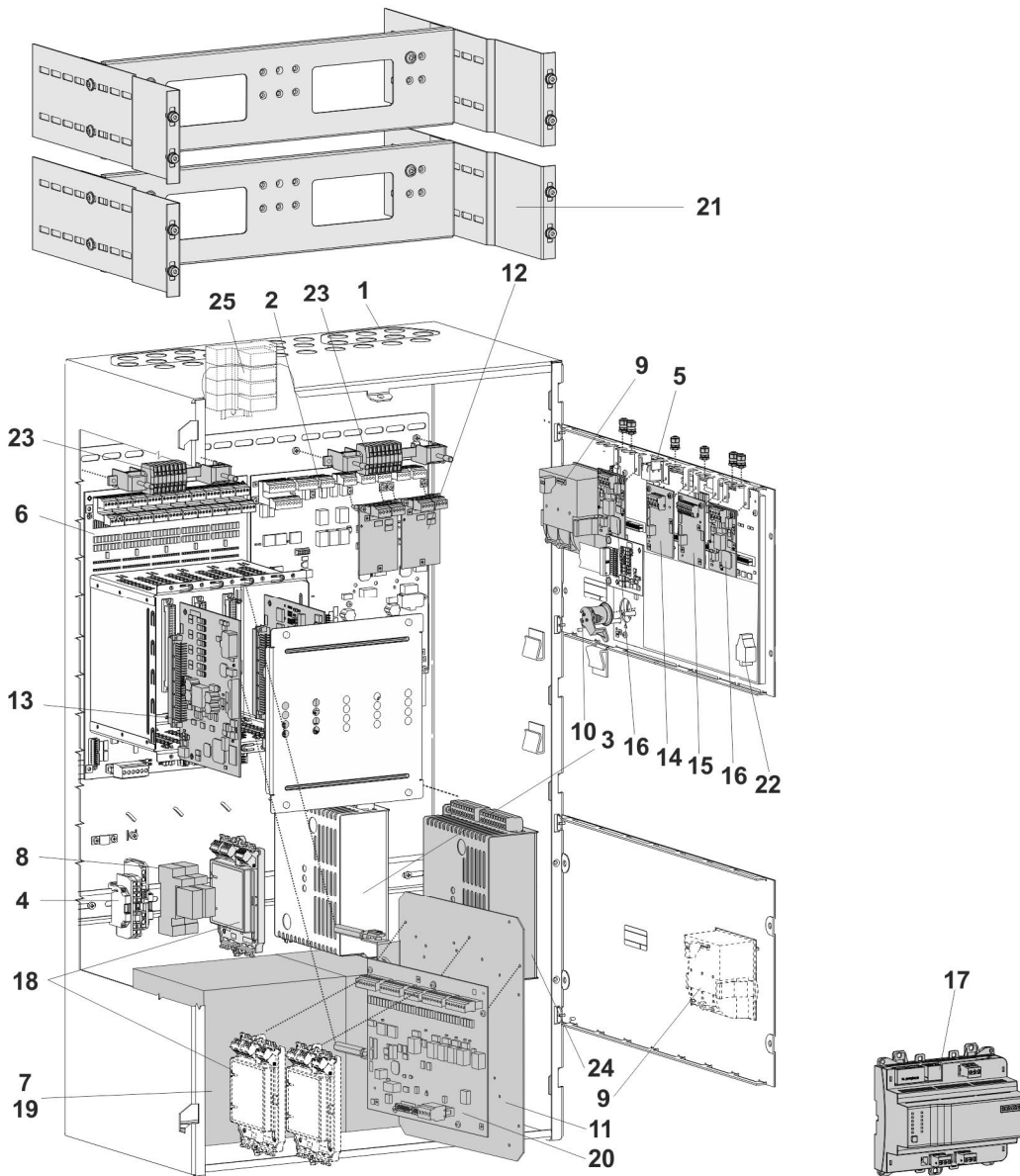
Fig. 4: Layout of FC726
