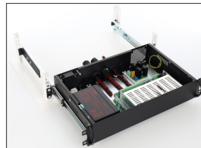
Mounting on a ARAS450N rail
