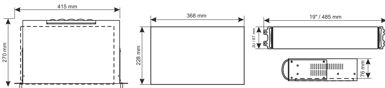
Mounting on a ARAS450N rail
