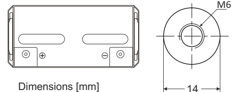
Pole terminals
